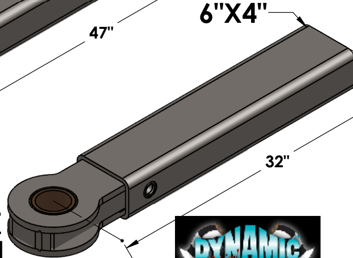
755 SHORT EXTENSION
